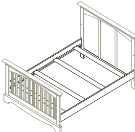
Ragusa Full-Size Bed Rails – 1216 W:59 x D:80 x H:46
